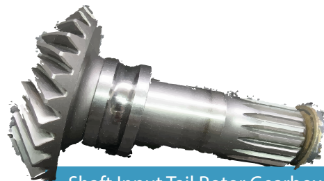
Shaft Input Tail Rotor Gearbox
